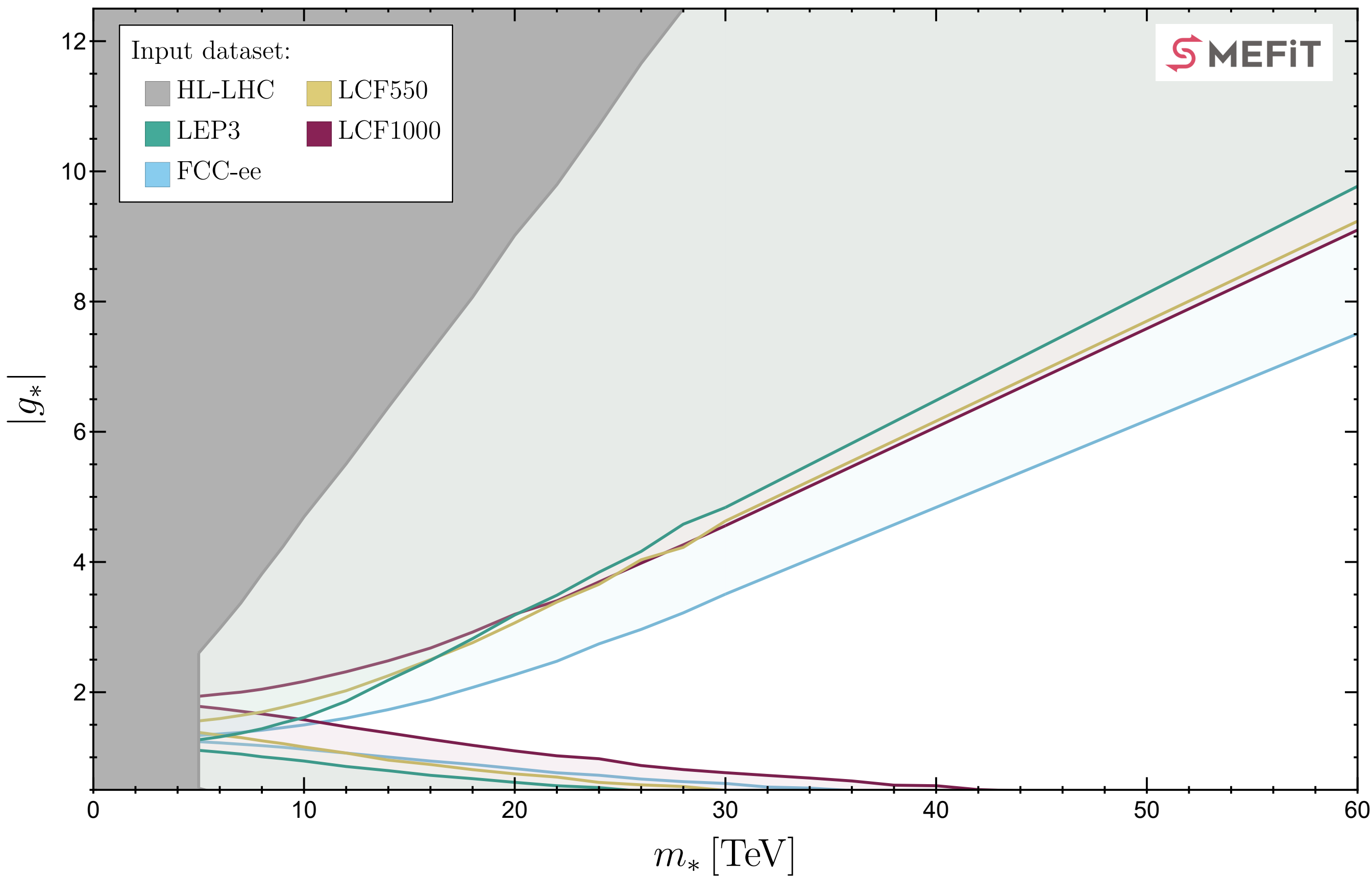
95% C.I. on Composite Higgs coupling
